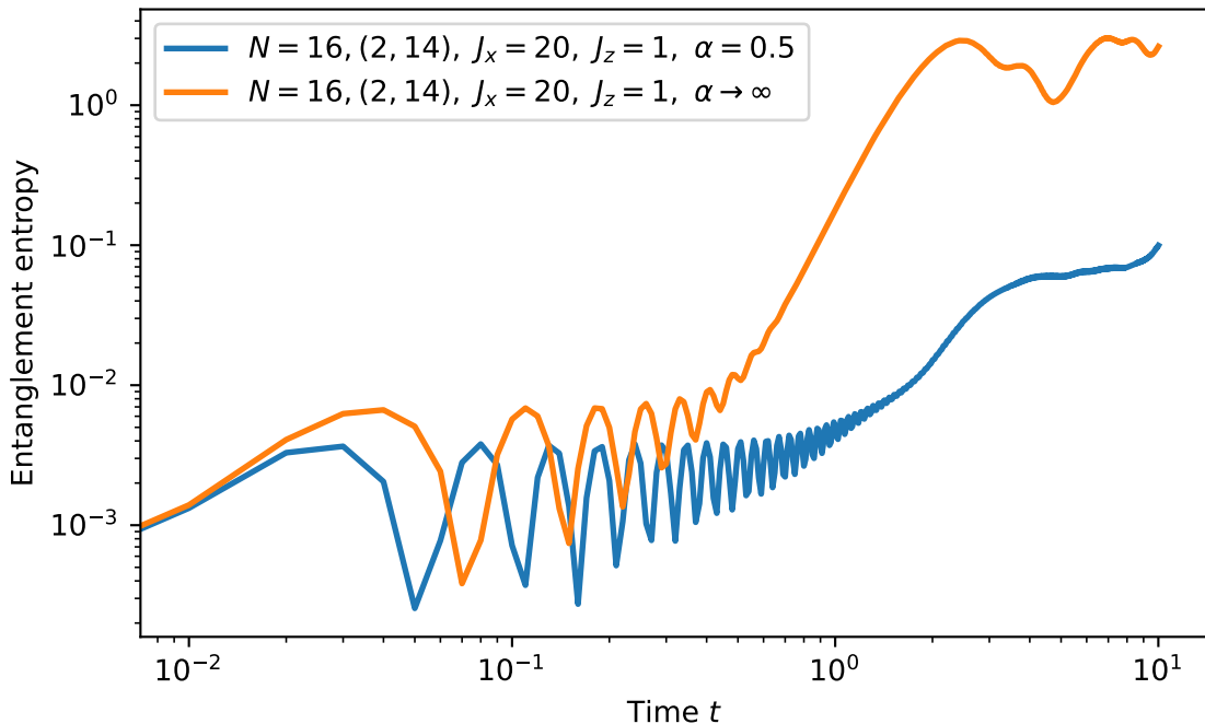
Half chain entanglement entropy(t)
